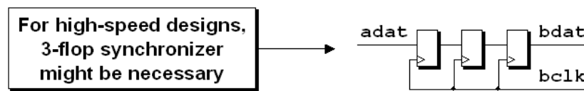
Figure 5 - Three flip-flop synchronizer used in higher speed designs
