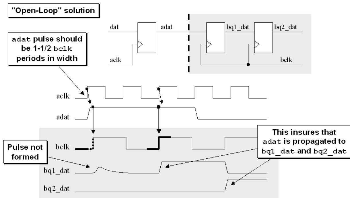
Figure 10 - Lengthened pulse to guarantee that the control signal will be sampled
