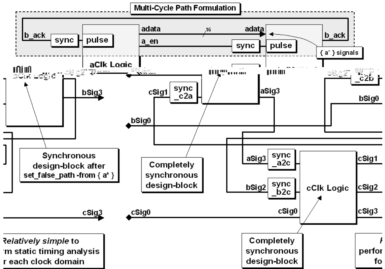
Figure 31 - Partitioned design with MCP formulation
